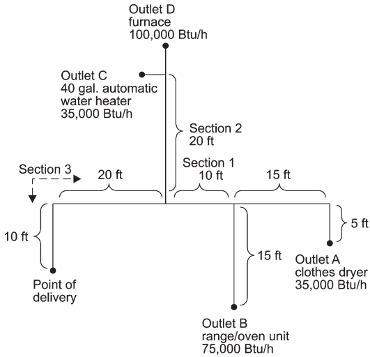
FIGURE A.7.1 PIPING PLAN SHOWING A STEEL PIPING SYSTEM
